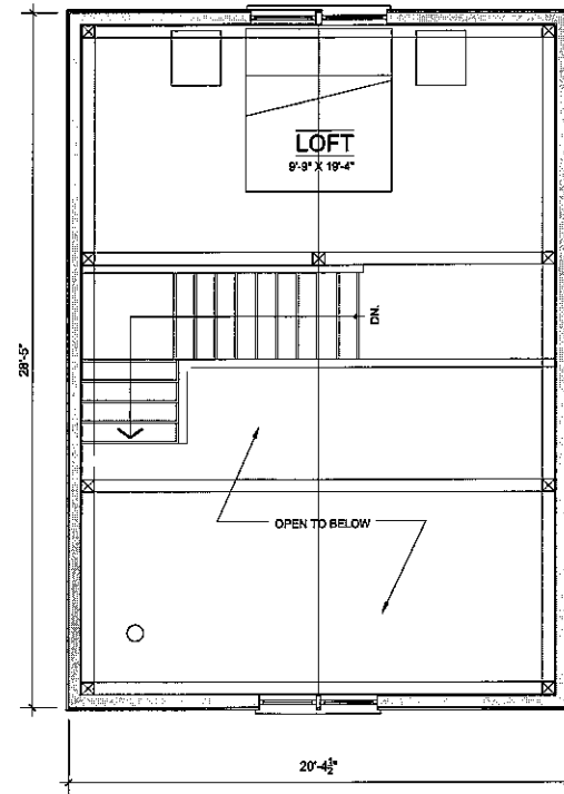
Proposed Loft Level
