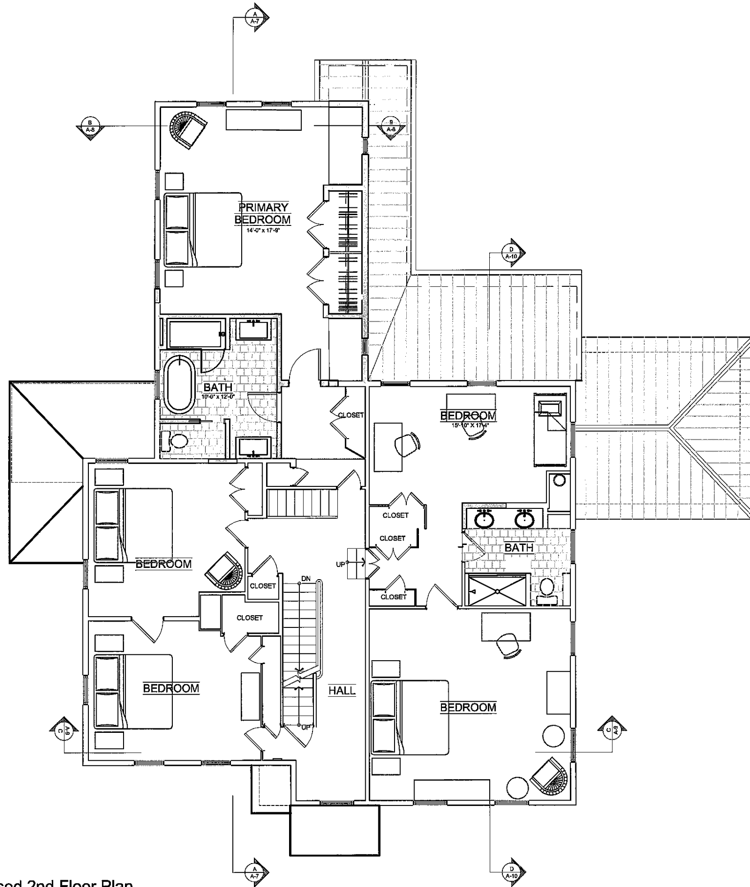
Proposed 2nd Floor Plan
