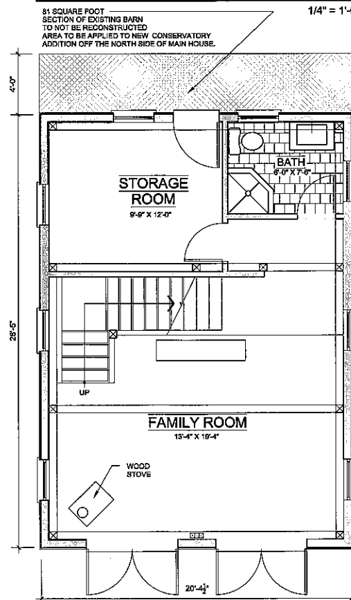
Proposed 1st Floor Plan
