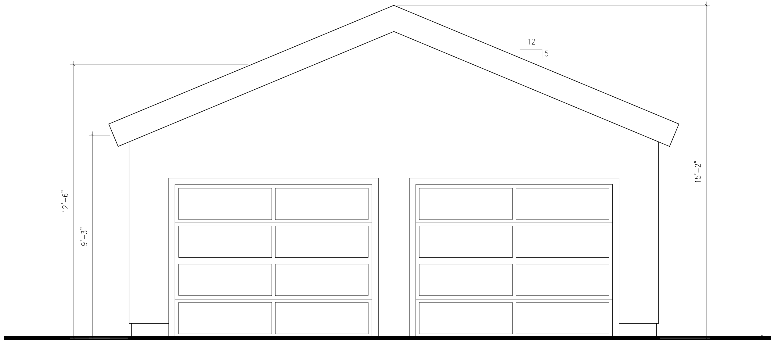
GARAGE FRONT ELEVATION W/ 5:12 PITCH
