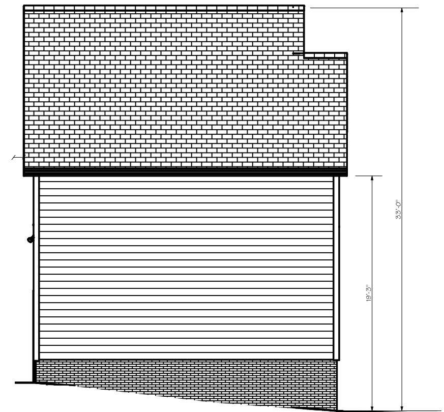
PROPOSED RIGHT ELEVATION SCALE: 1/8"=1'-0"
