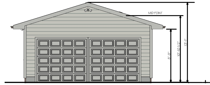
EXIST. FRONT ELEVATION SCALE: 1/8"=1'-0"
