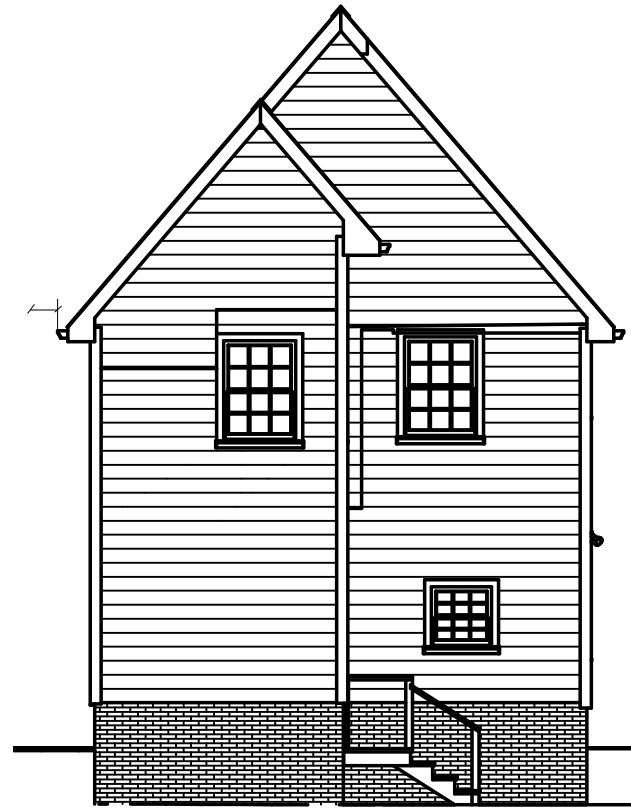
PROPOSED REAR ELEVATION SCALE: 1/8"=1'-0"
