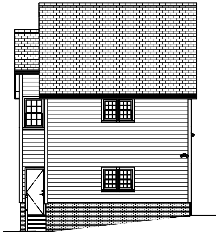
PROPOSED LEFT ELEVATION SCALE: 1/8"=1'-0"
